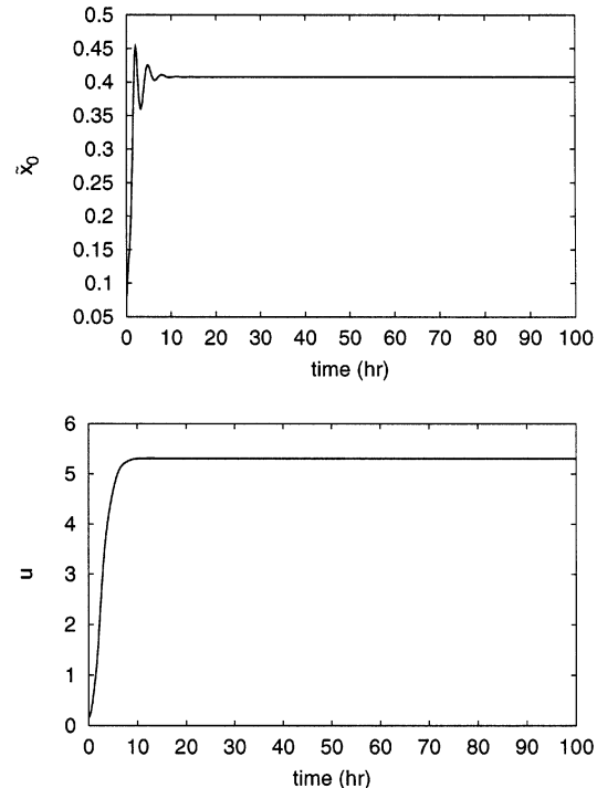
Figure 4. Controlled output (crystal concentration) and manipulated input (solute concentration) for crystallizer moment model under bounded nonlinear controller with constrained process input in [0, 6] and initial condition inside closed-loop stability region.
