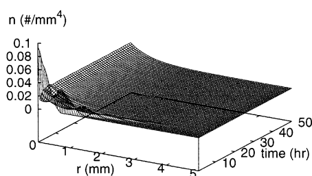
Figure 7. Controlled output (crystal concentration), manipulated input (solute concentration), and crystal-size distribution for crystallizer process model of Eq. 4 under bounded nonlinear controller (solid line) and PI controller (dashed line) for 0.4 increase in the set point with input constraints u \in [0, 6] and 5% modeling error in both F and \tau .
