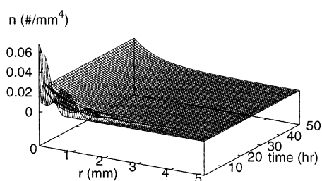
Figure 6. Controlled output (crystal concentration), manipulated input (solute concentration), and crystal-size distribution for crystallizer process model of Eq. 4 under bounded nonlinear controller (solid line) and PI controller (dashed line) for 0.4 increase in the set point and u \in [0, 6] .
